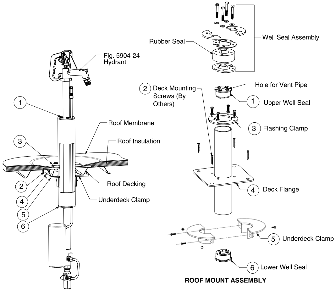
Installation Illustration (For Illustration Purpose Only)
