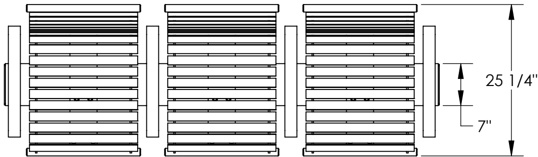
TOP VIEW
