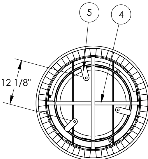
BOTTOM VIEW MOUNTING DETAIL
