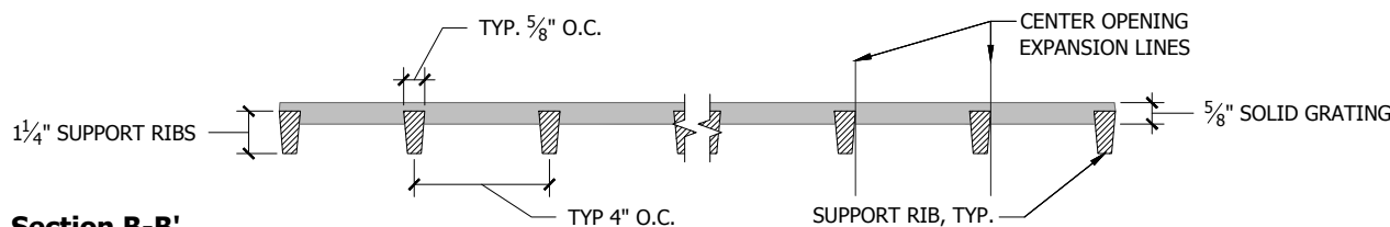
Section B-B'
